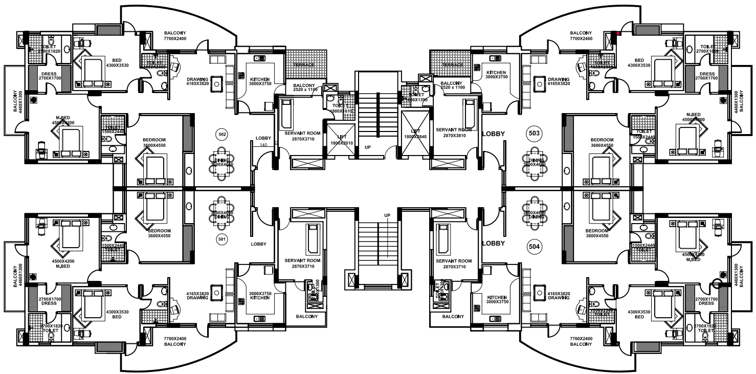
5th FLOOR PLAN
